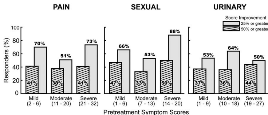
Improvement in pain, urinary and sexual scores after therapy, as assessed by PPSS
